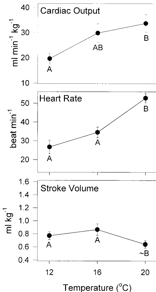
FIGURE 1.—Influence of temperature on resting values for cardiac parameters of smallmouth bass. Scales for y-axes are relative to (i.e., 0.5\times to 2.1\times ) the 12°C values. Fish were acclimated for more than 4 weeks at 12°C ( n = 8 ), 16°C ( n = 9 ), and 20°C ( n = 14 ). Points within a panel with different letters were significantly ( \sim = marginally) different.
