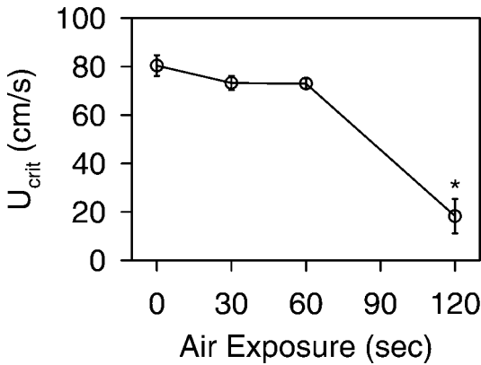
FIGURE 1.—Swimming performance, measured as critical swimming speed ( U_{crit} ; mean \pm SE), of brook trout chased by hand for 30 s and subjected to 0-, 30-, 60-, and 120-s air exposures. The asterisk indicates a significant difference. The duration of air exposure had a significant effect on swimming performance ( P < 0.001 ). However, only the 120-s treatment showed a significant decrease ( P < 0.001 ). The 30- and 60-s treatments were not significantly different than controls when the 120-s treatment was removed from the analysis.
